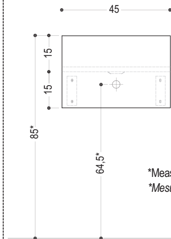
Front view - Vue frontale
