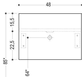
Front view - Vue frontale
