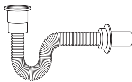
S5 Chrome flexible pipe Ø32 mm with Ø32 or Ø40 mm connection. Max length 500 mm. Tube flexible Ø32 mm avec Ø32 or Ø40 mm raccordement. Longeur max. 500 mm.
